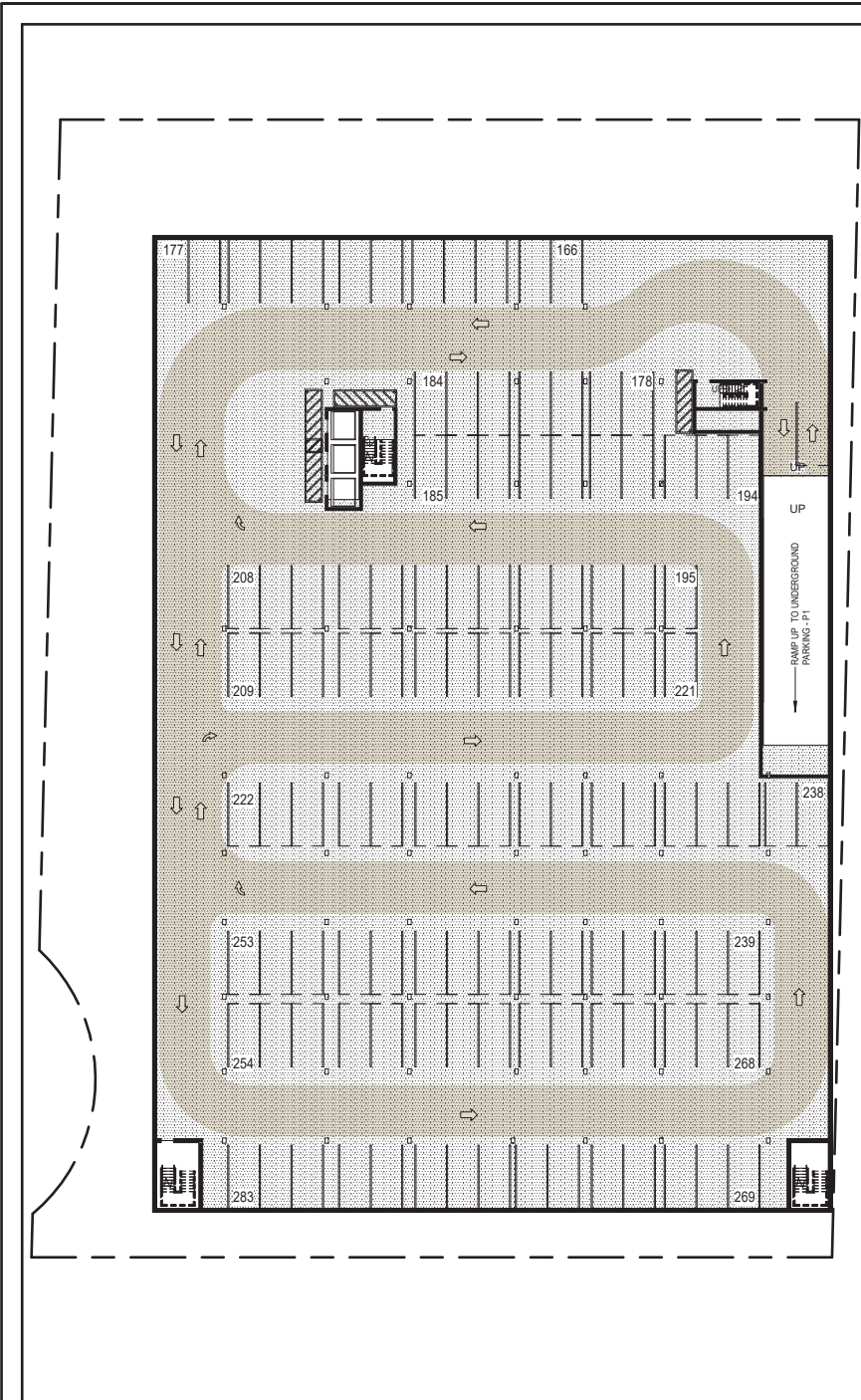
2 UNDERGROUND PARKING - P2 A3 1 : 300
