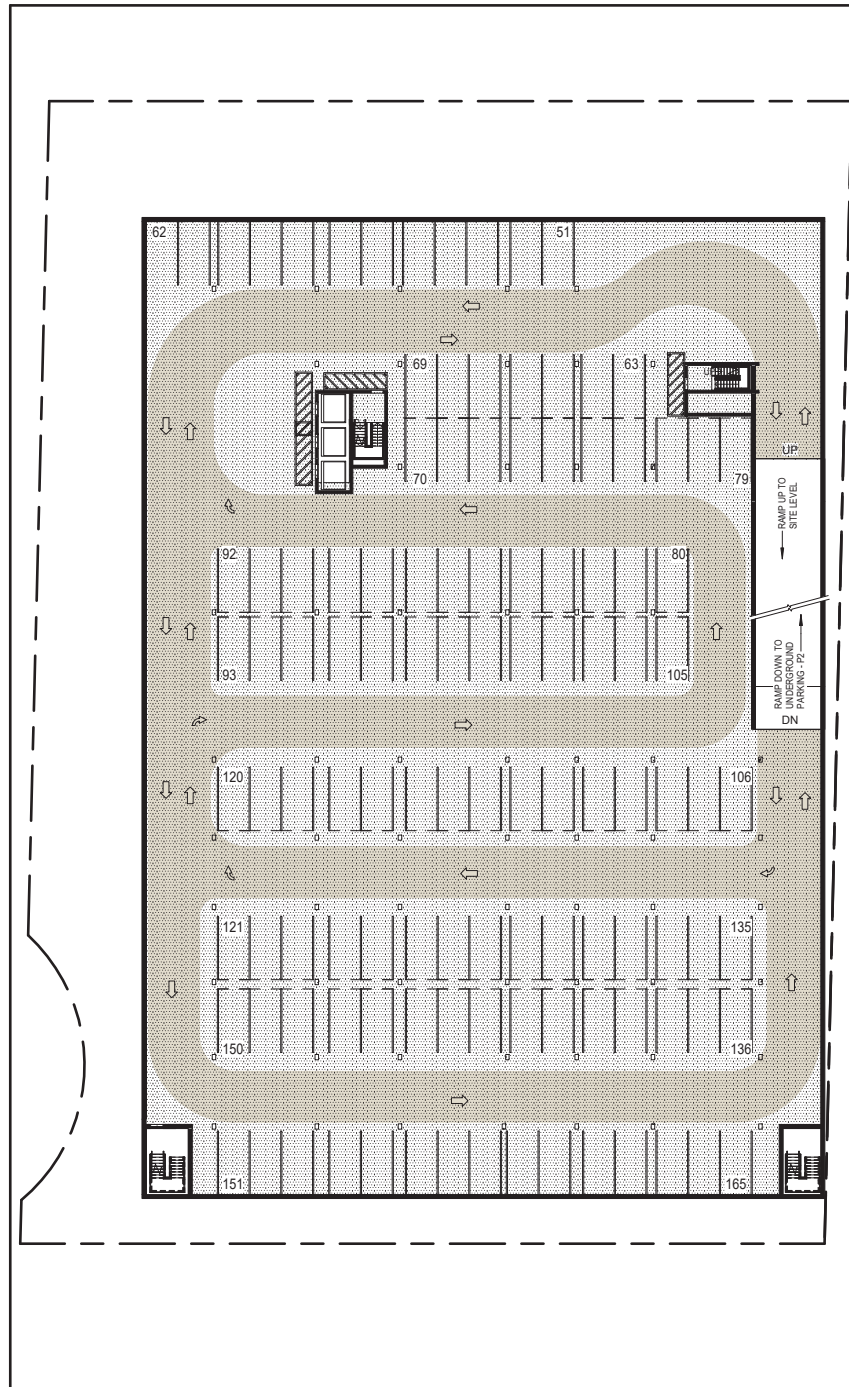
1 UNDERGROUND PARKING - P1 A3 1 : 300
