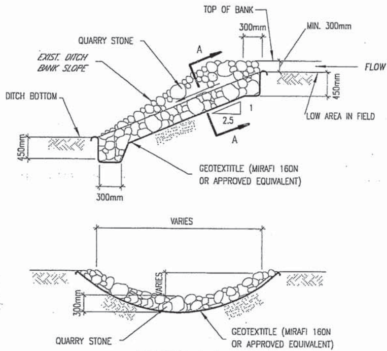
SECTION A-A TYPICAL ROCK CHUTE
