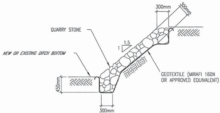
TYPICAL DITCH BANK RIP-RAP
