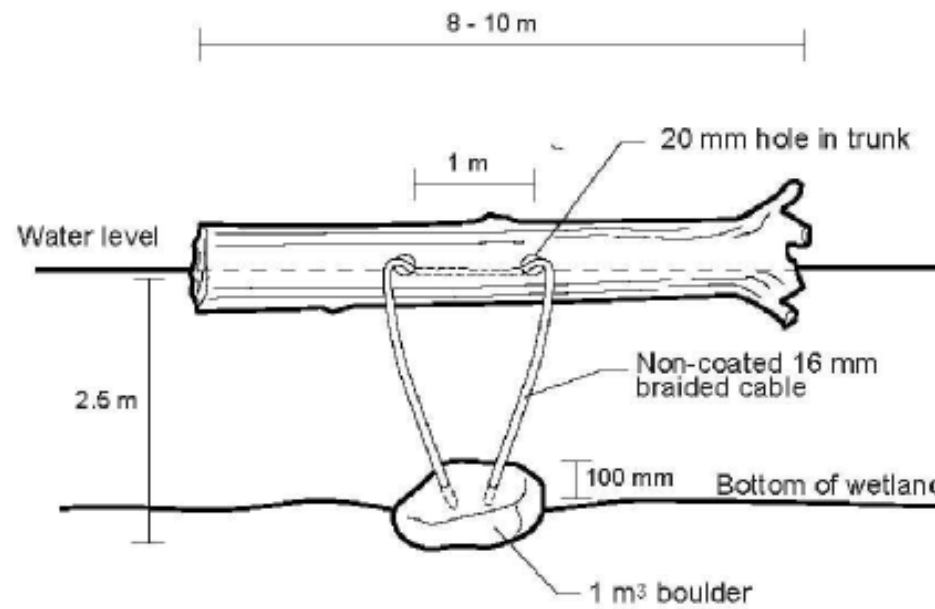
Detail: Floating Basking Log
