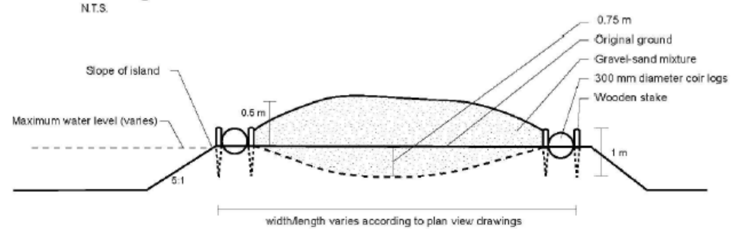
Detail: Turtle Nesting Island
