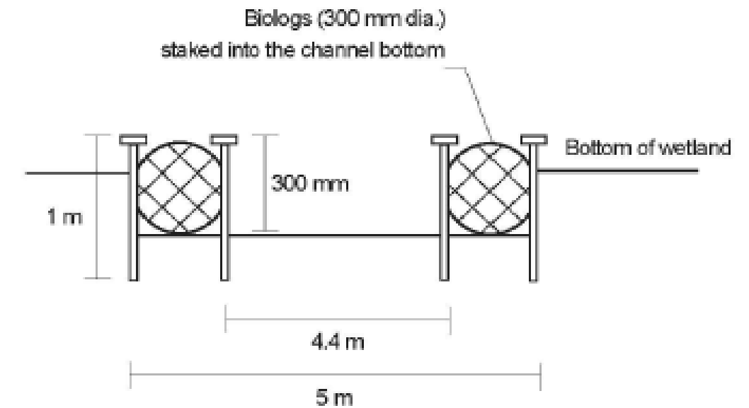
Cross Section: Drainage Channel
