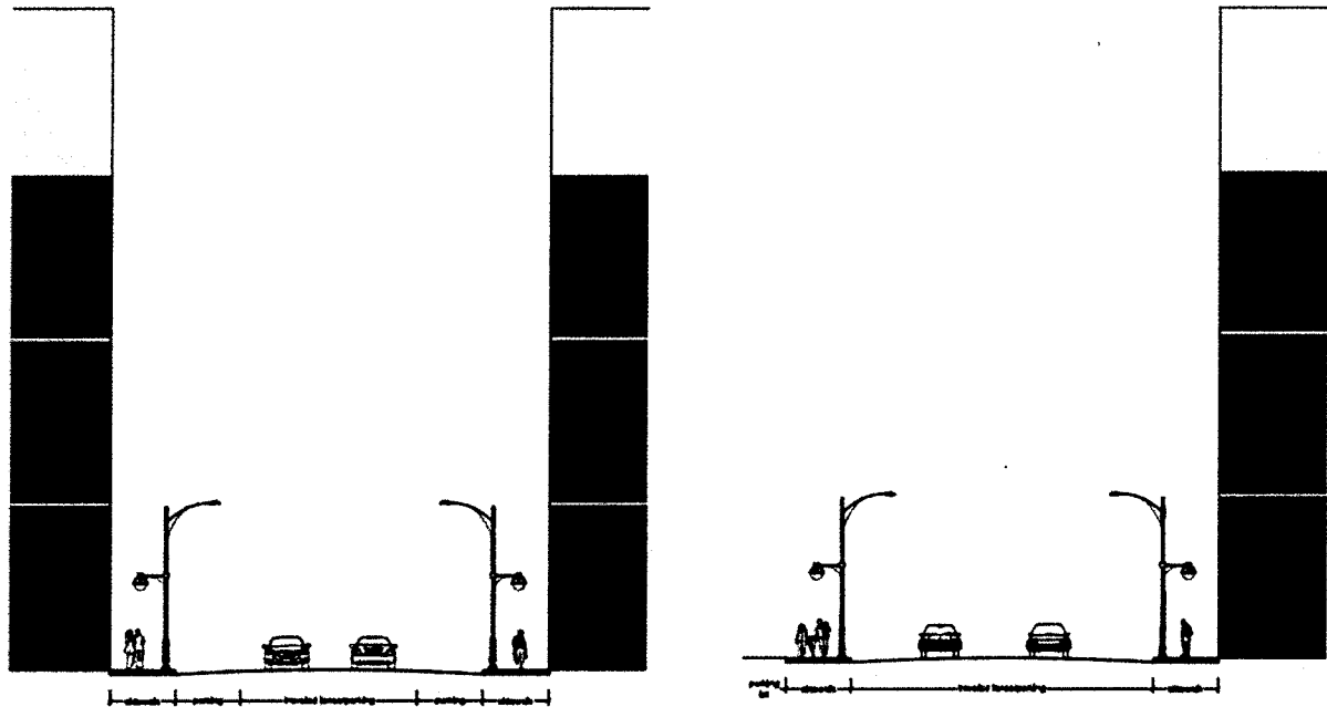
Section D-D Typical Commercial Street Profile Fullarton Street
