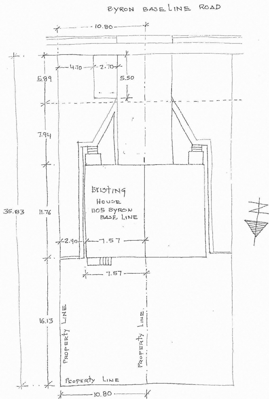
PROPOSED SITE PLAN Escale: 1:200 AP.
